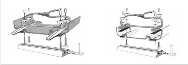
Fitting Kits for roof boxes with Comfort Sliding Fitting or Simple Sliding Fitting, e.g. Delphin, Topstar, Husky
