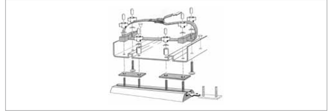
Fitting Kits for roof boxes with fixed drilling (50 mm interval)
