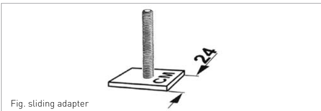
Fitting Kit for Fig. 2 Comfort Sliding Fitting
